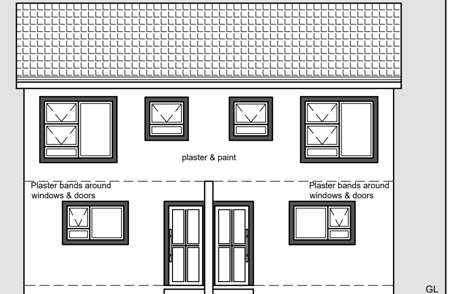
REAR ELEVATION
